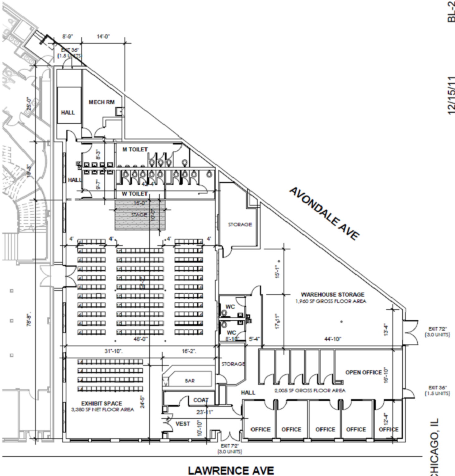
1 FLOOR PLAN 1" = 20'-0"
